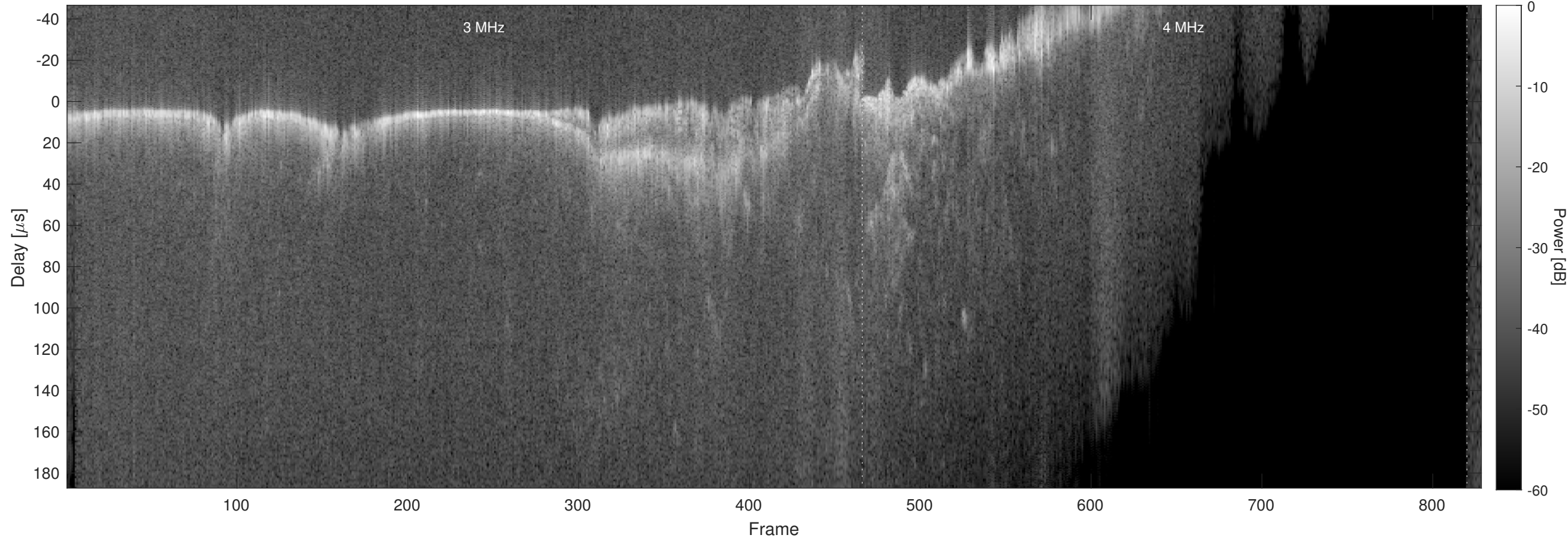
Orbit 9693, Chapman, No Window, Channel 2
