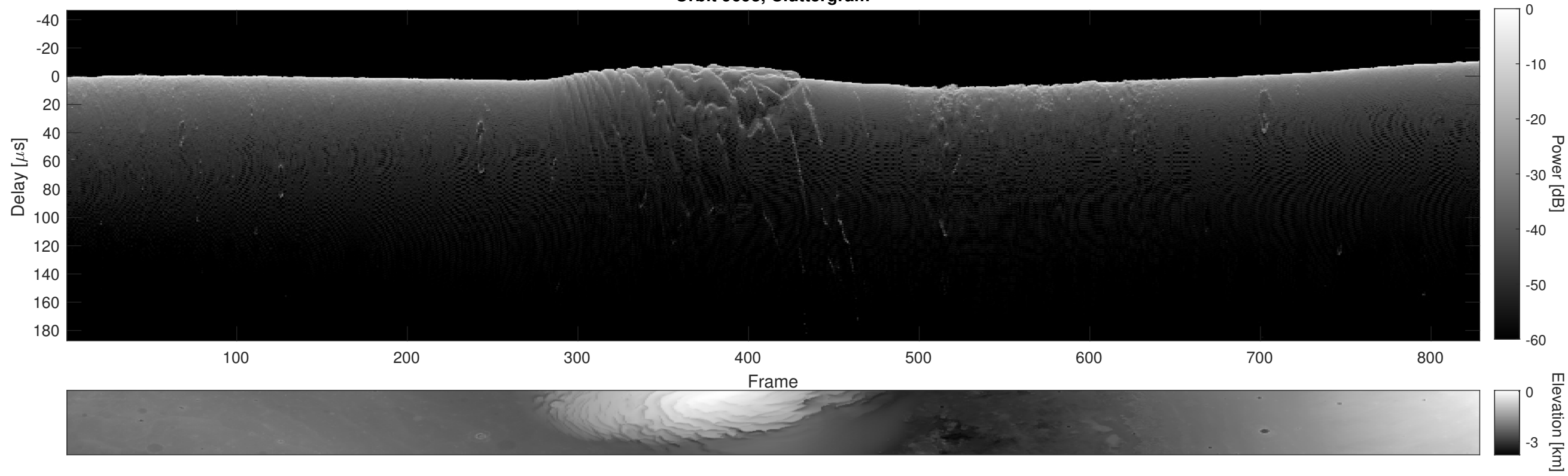
Orbit 9693, Cluttergram
