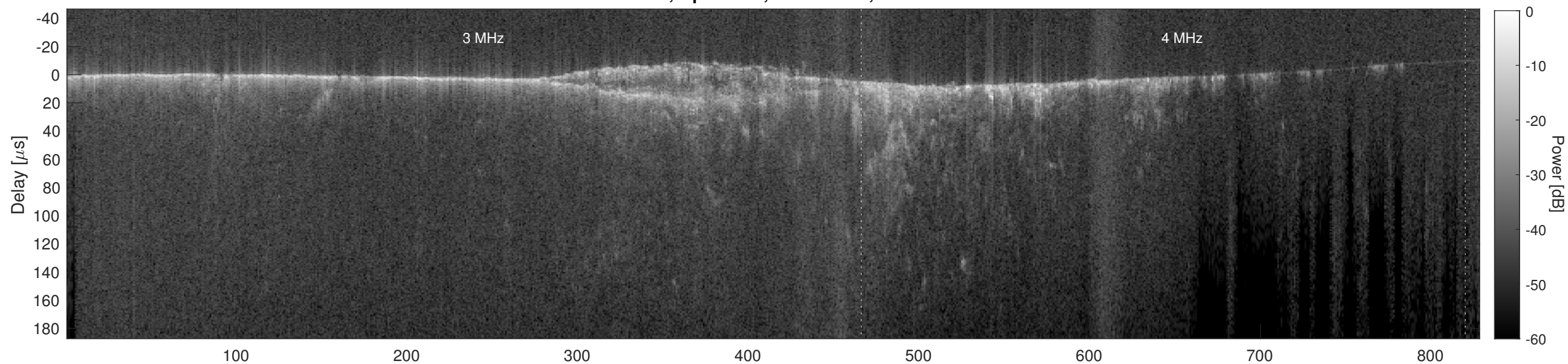
Orbit 9693, Cluttergram
