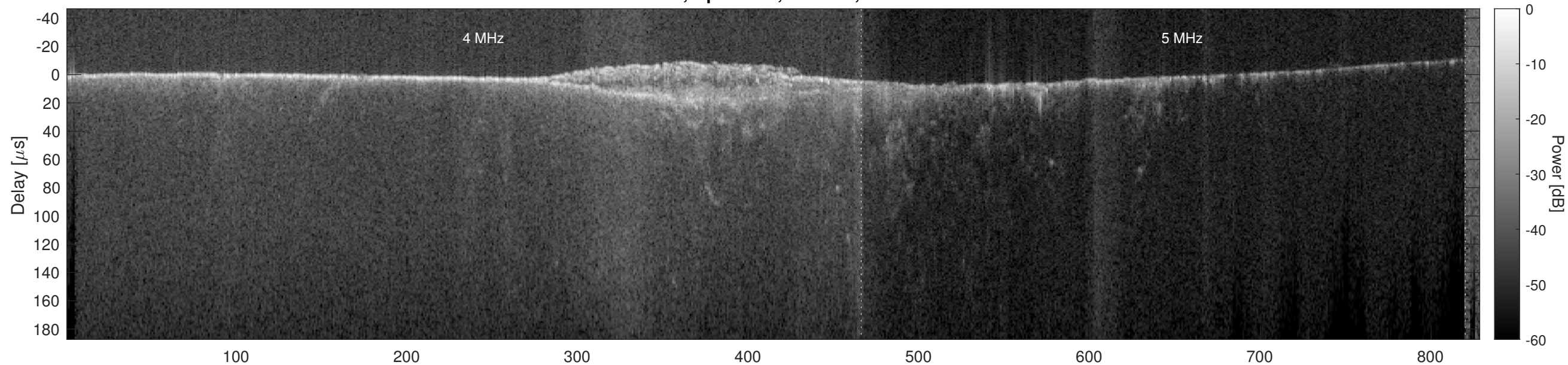
Orbit 9693, Optimized, Window, Channel 2
