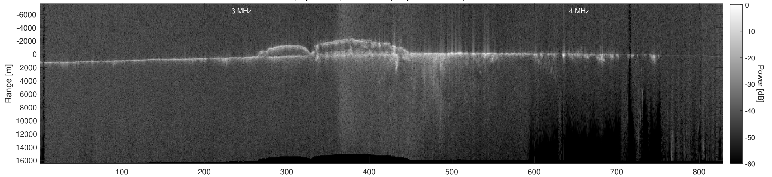
Orbit 9694, Depth-Corrected Cluttergram
