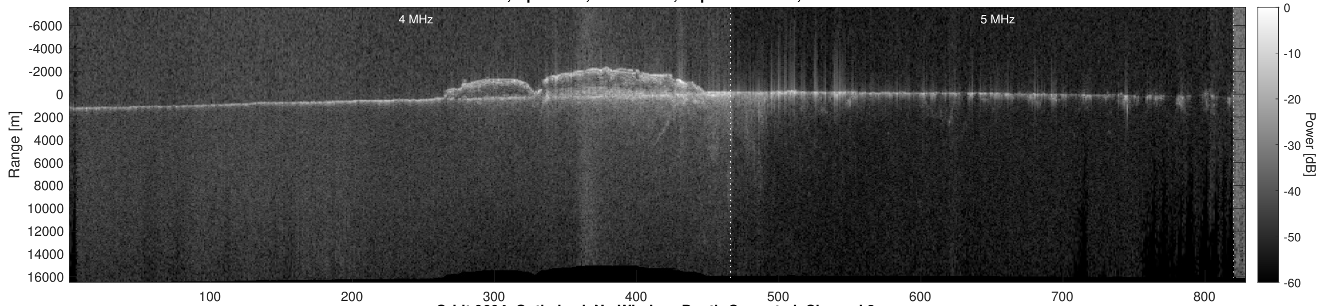
Orbit 9694, Optimized, No Window, Depth-Corrected, Channel 2
