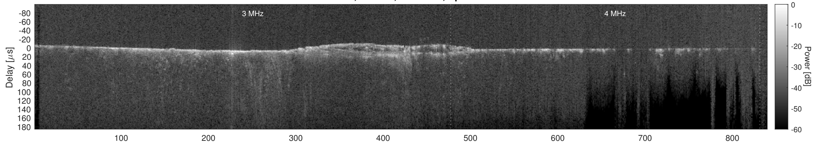
Orbit 9695, Cluttergram
