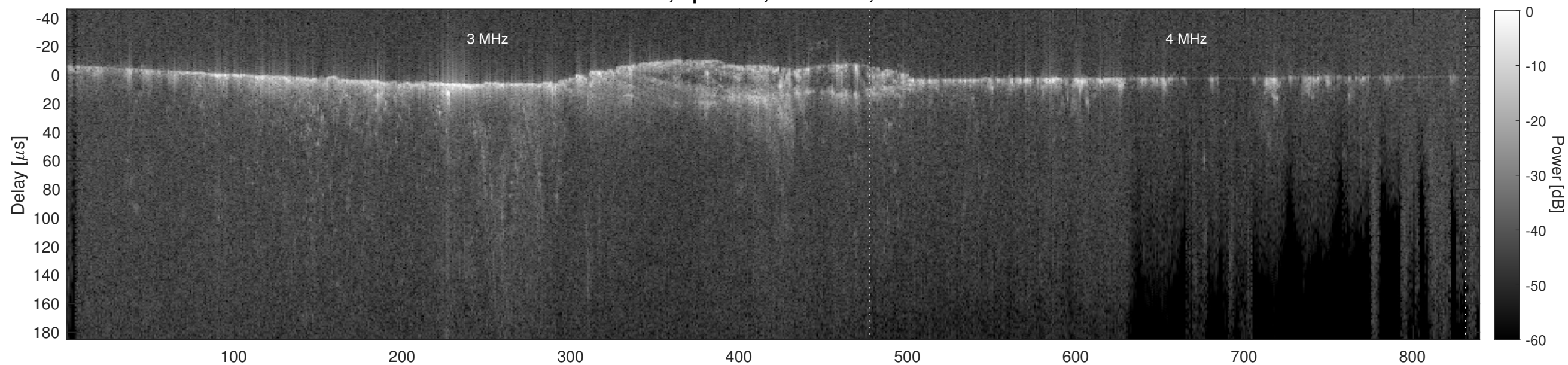
Orbit 9695, Cluttergram
