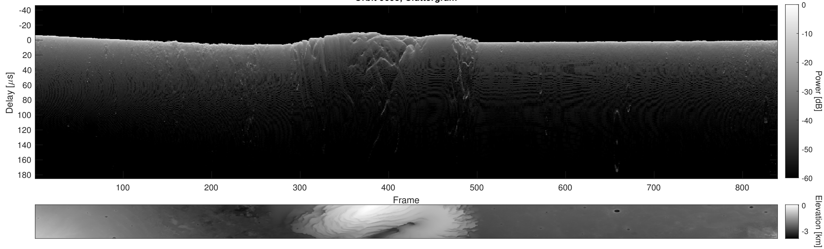
Orbit 9695, Cluttergram
