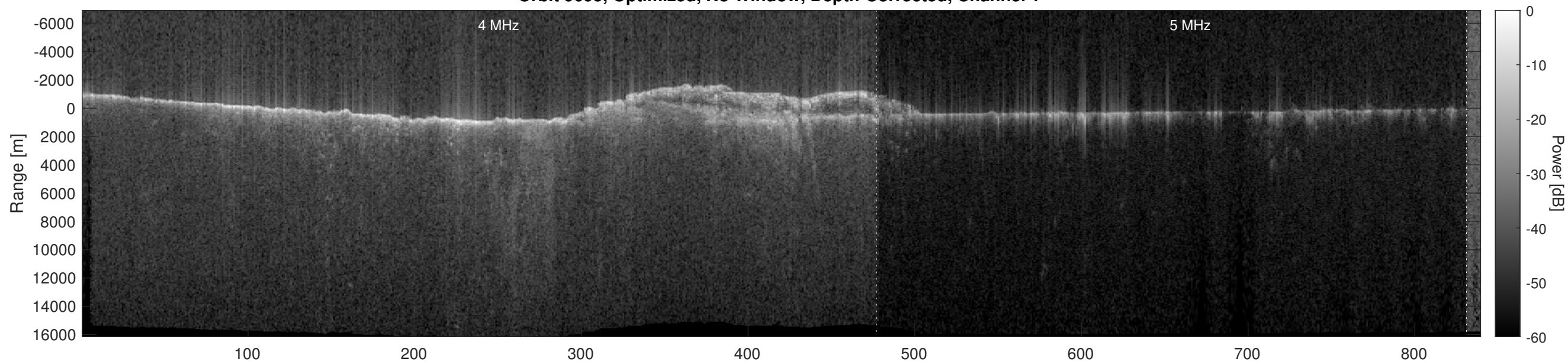
Orbit 9695, Optimized, No Window, Depth-Corrected, Channel 2
