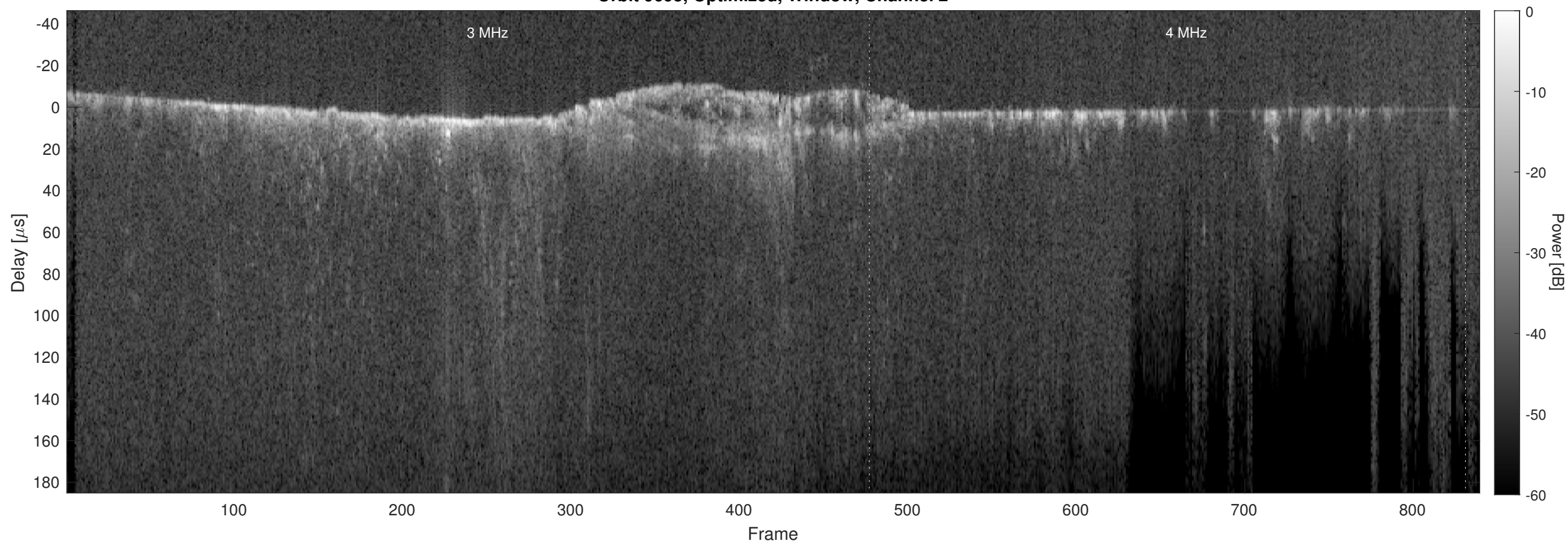
Orbit 9695, Optimized, Window, Channel 2
