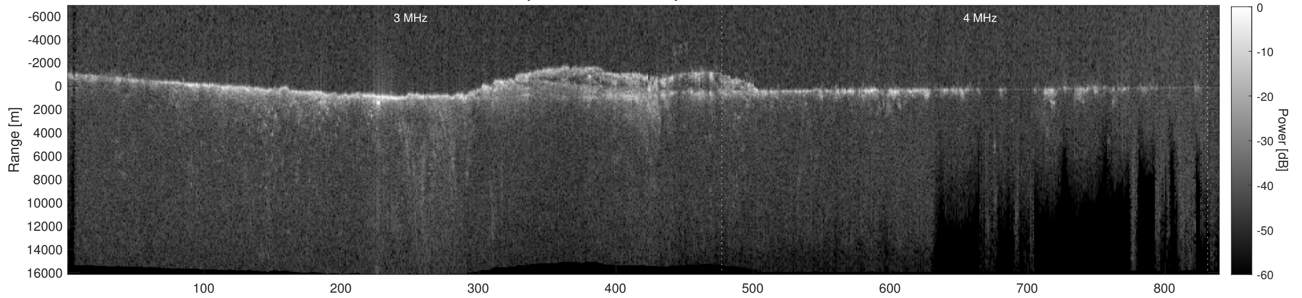
Orbit 9695, Depth-Corrected Cluttergram
