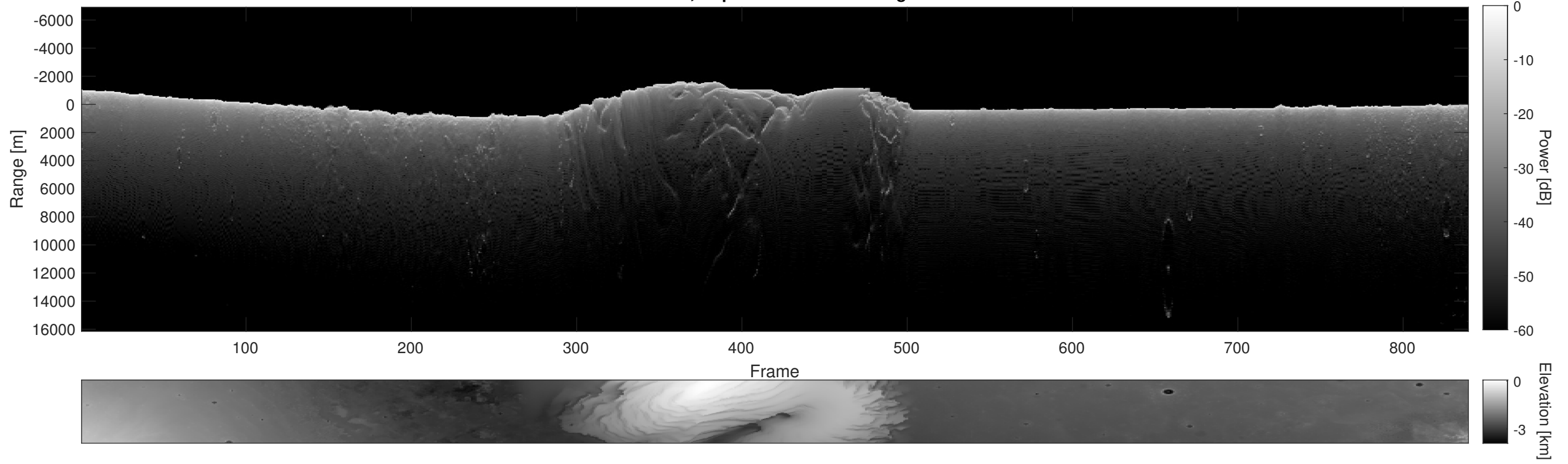
Orbit 9695, Depth-Corrected Cluttergram
