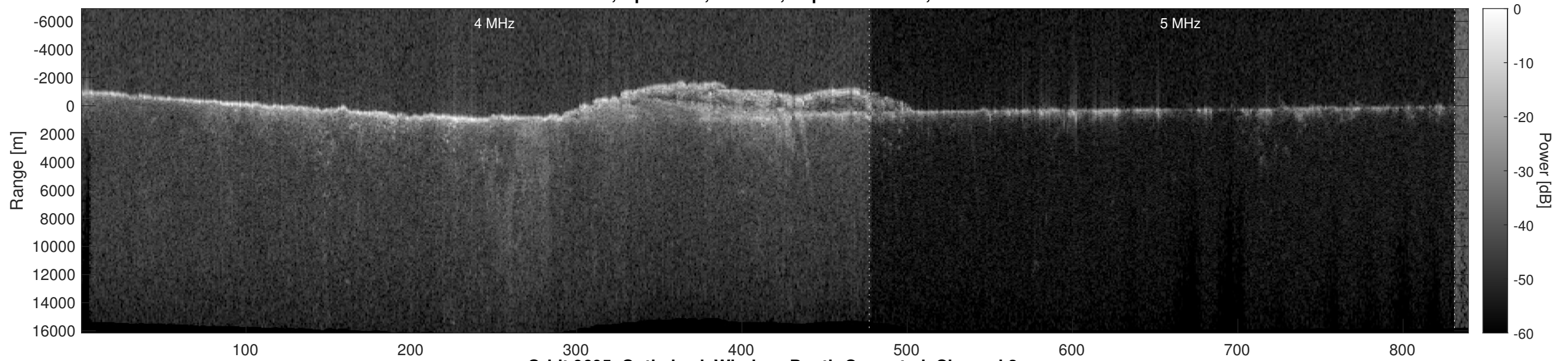
Orbit 9695, Optimized, Window, Depth-Corrected, Channel 2
