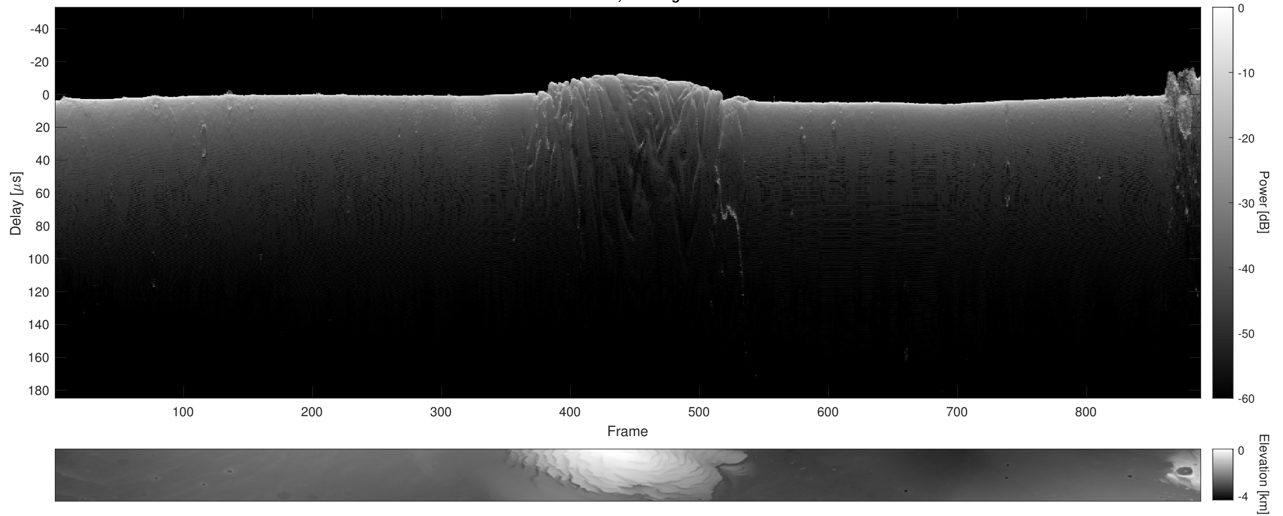
Orbit 9696, Cluttergram
