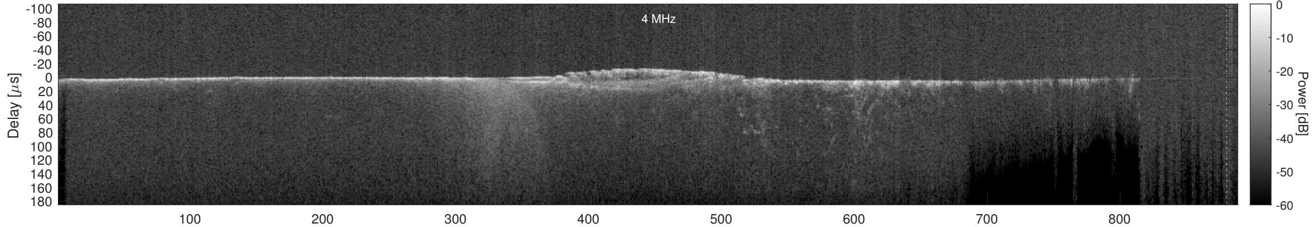
Orbit 9696, Cluttergram
