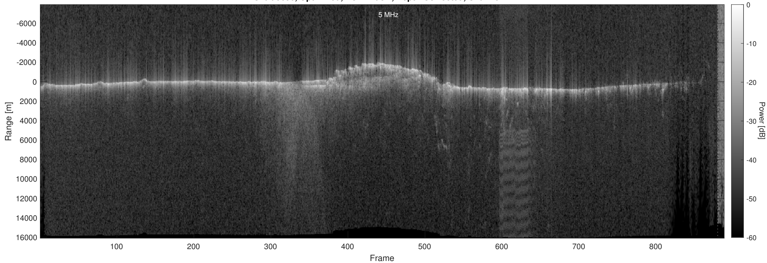
Orbit 9696, Optimized, No Window, Depth-Corrected, Channel 2
