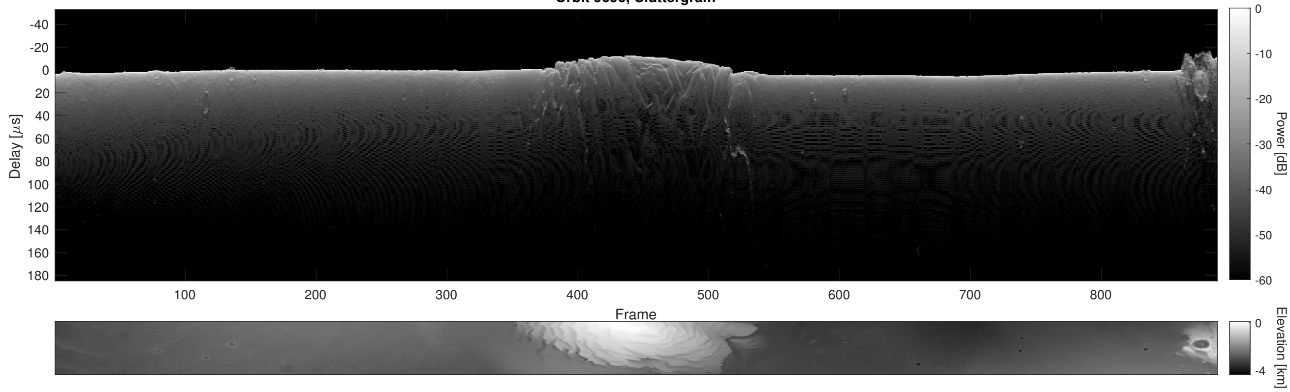
Orbit 9696, Cluttergram
