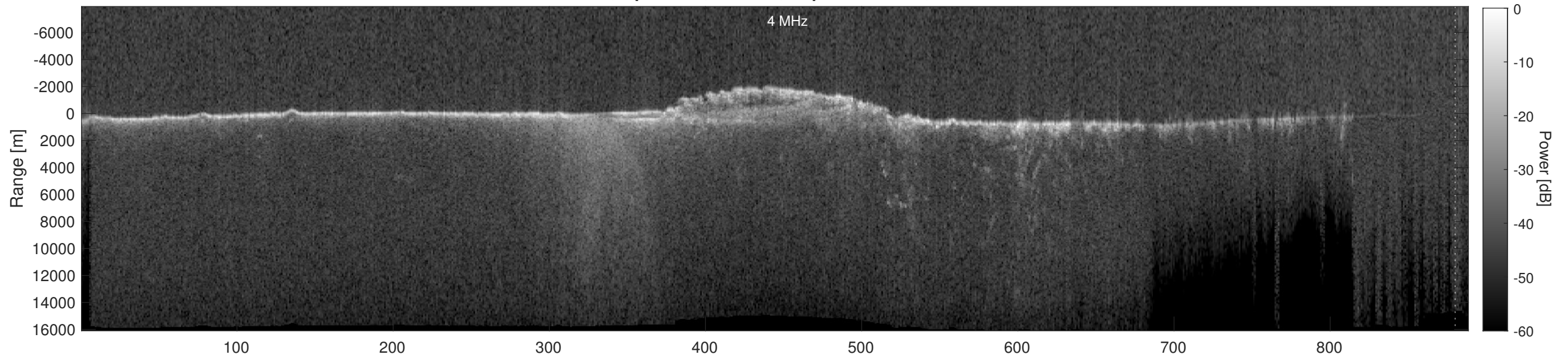
Orbit 9696, Depth-Corrected Cluttergram
