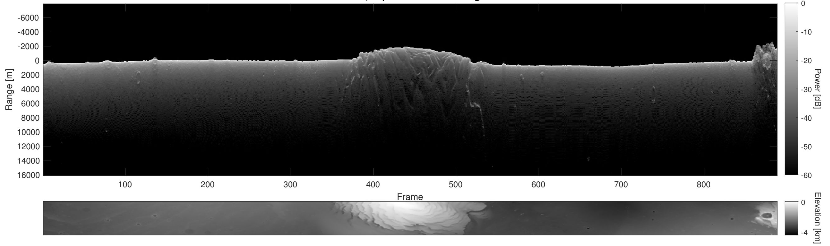
Orbit 9696, Depth-Corrected Cluttergram
