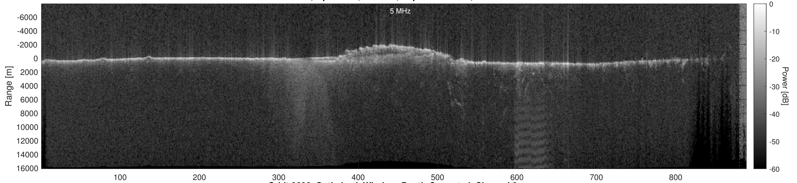
Orbit 9696, Optimized, Window, Depth-Corrected, Channel 2
