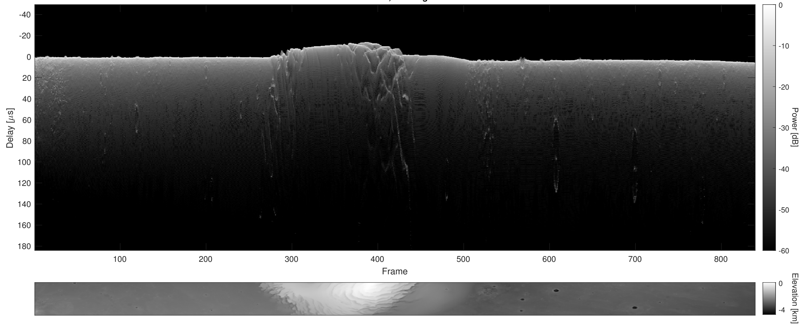
Orbit 9697, Cluttergram
