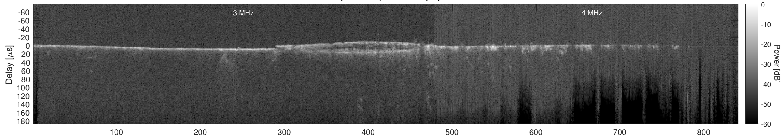
Orbit 9698, Cluttergram
