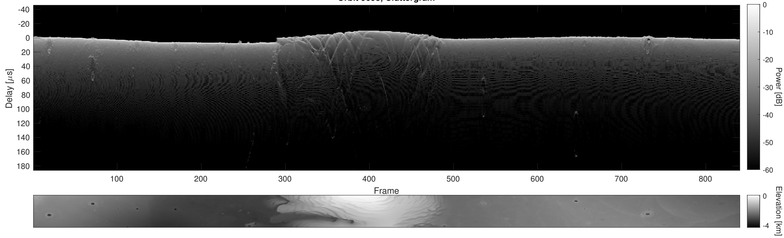
Orbit 9698, Cluttergram
