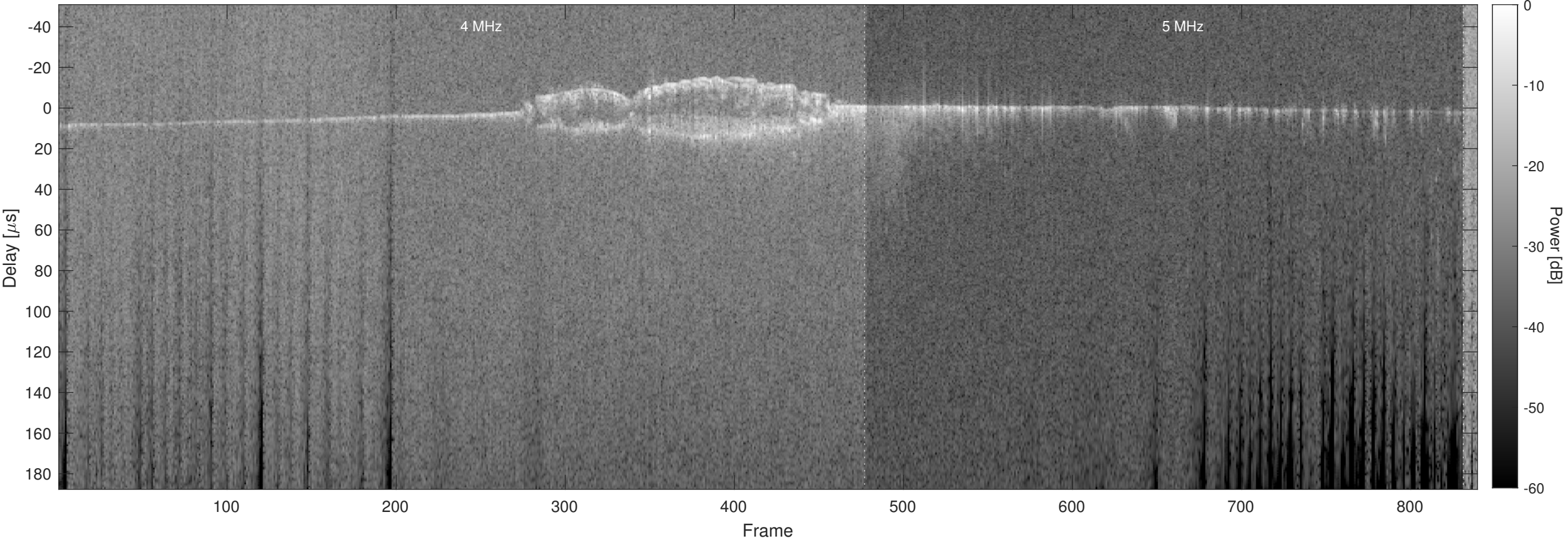
Orbit 9701, Optimized, No Window, Channel 2
