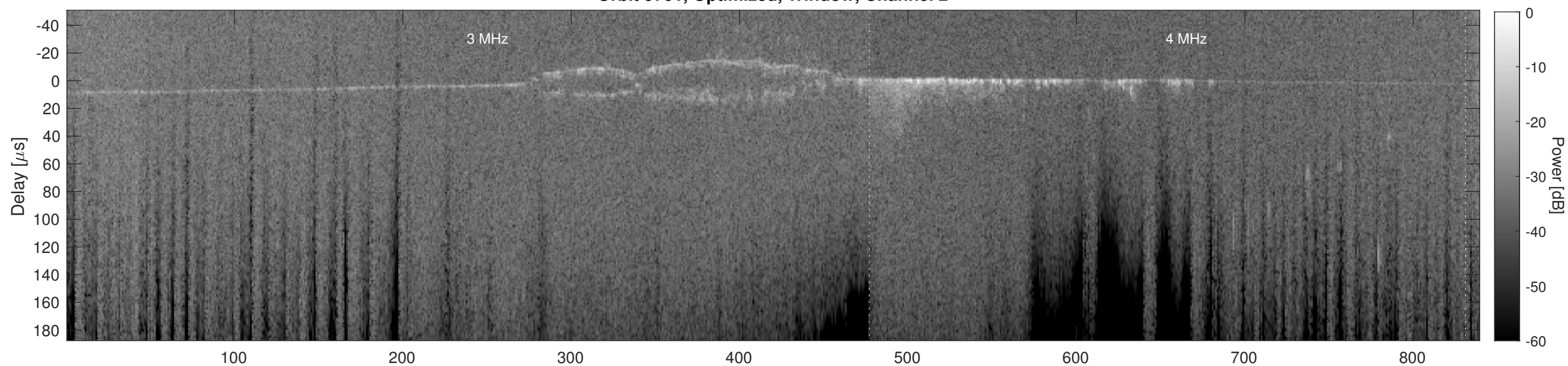
Orbit 9701, Cluttergram
