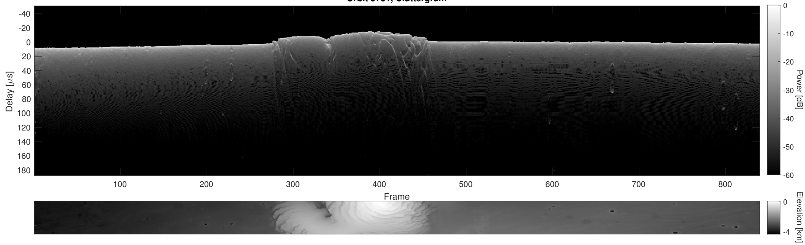
Orbit 9701, Cluttergram
