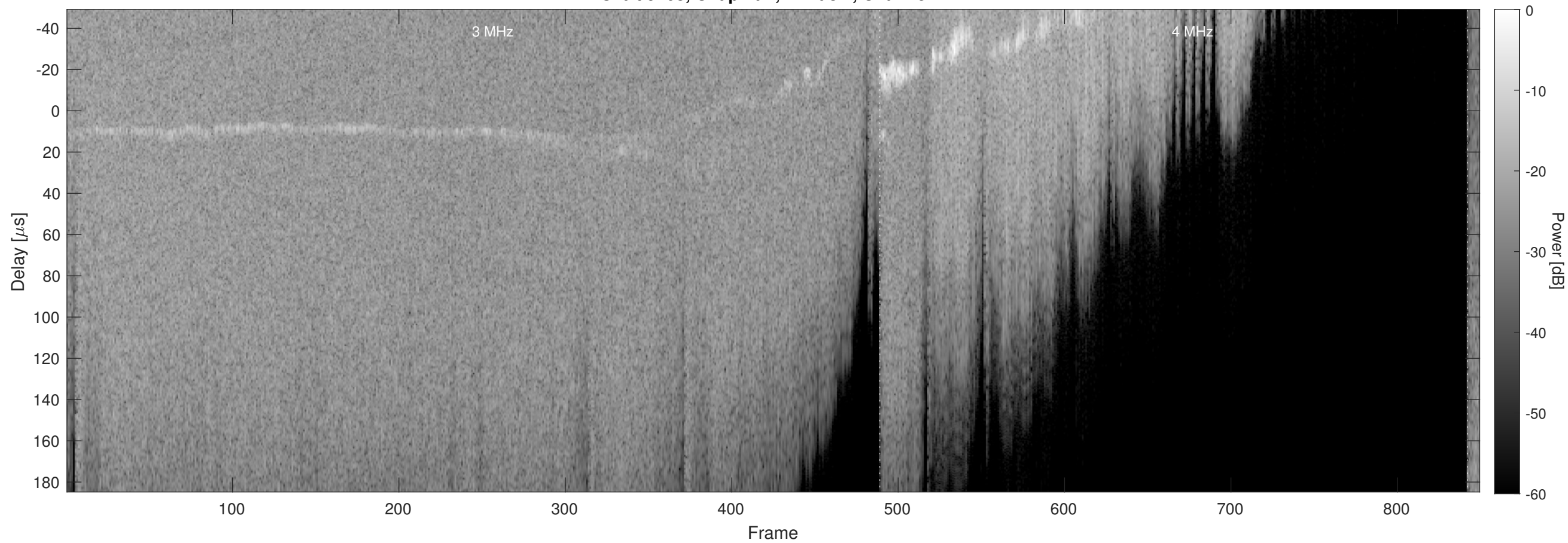
Orbit 9703, Chapman, Window, Channel 2
