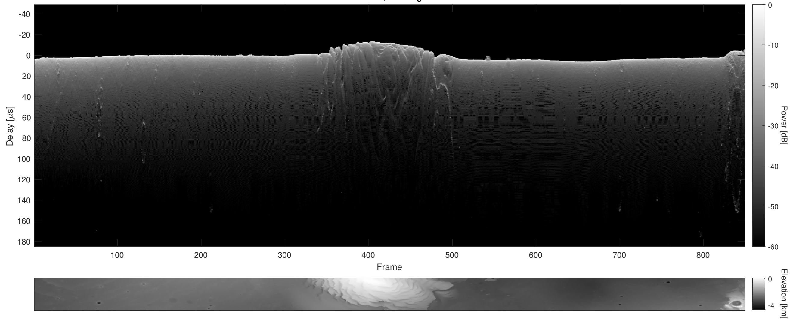
Orbit 9703, Cluttergram
