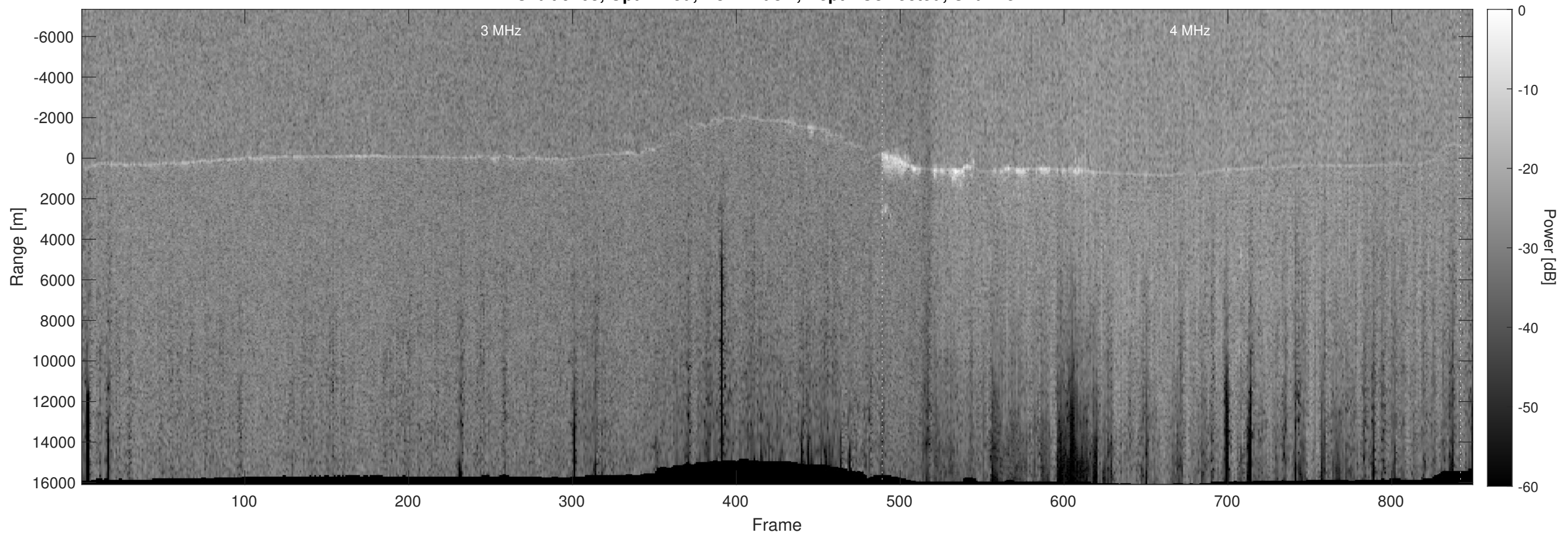
Orbit 9703, Optimized, No Window, Depth-Corrected, Channel 2
