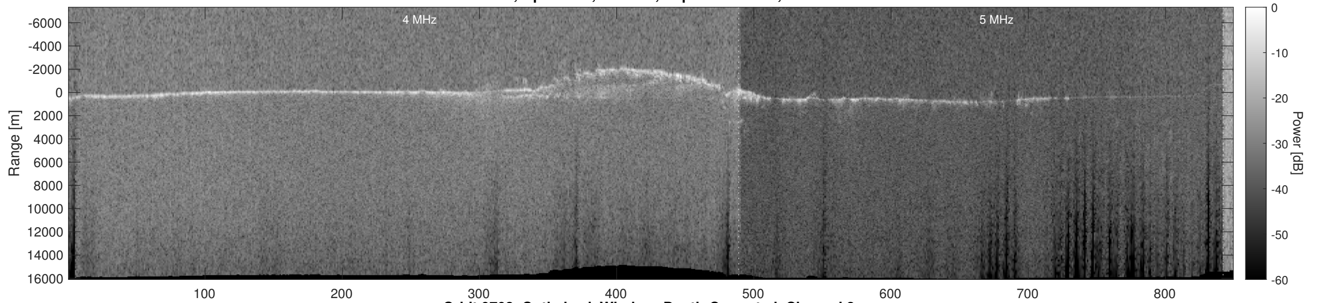
Orbit 9703, Optimized, Window, Depth-Corrected, Channel 2
