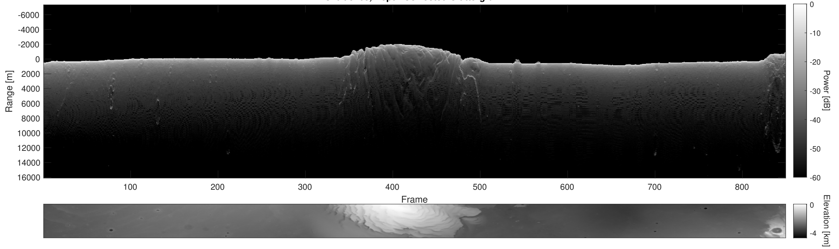
Orbit 9703, Depth-Corrected Cluttergram
