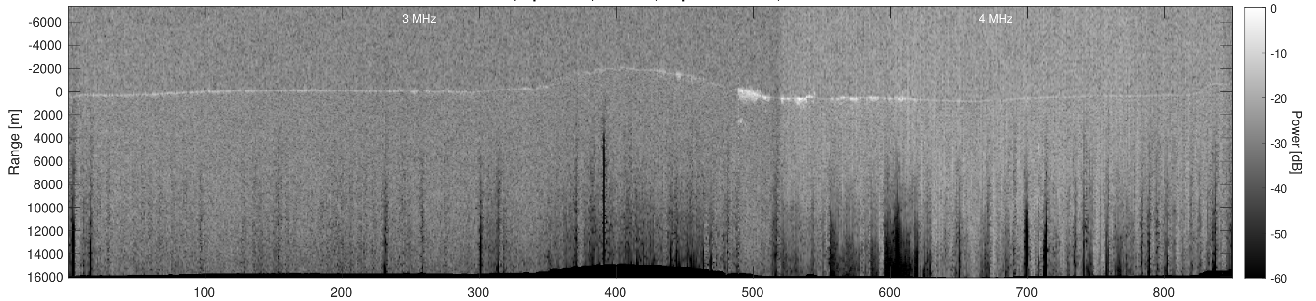
Orbit 9703, Depth-Corrected Cluttergram
