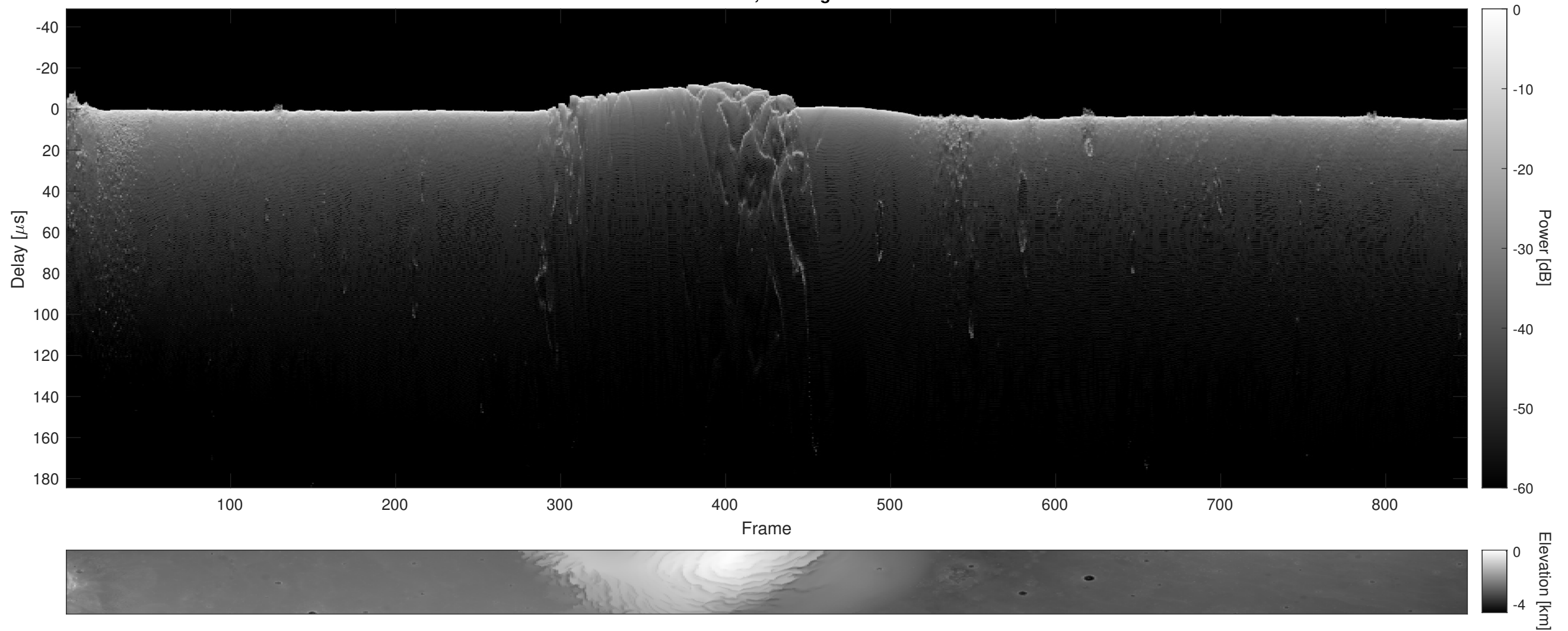
Orbit 9704, Cluttergram
