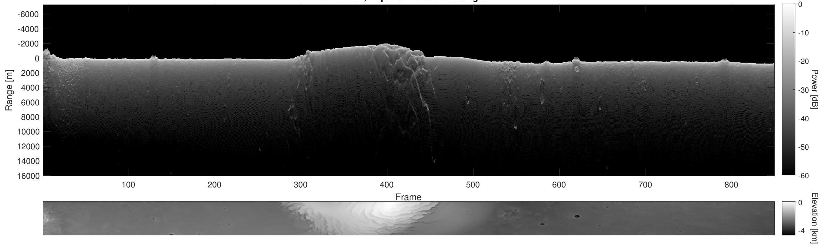
Orbit 9704, Depth-Corrected Cluttergram
