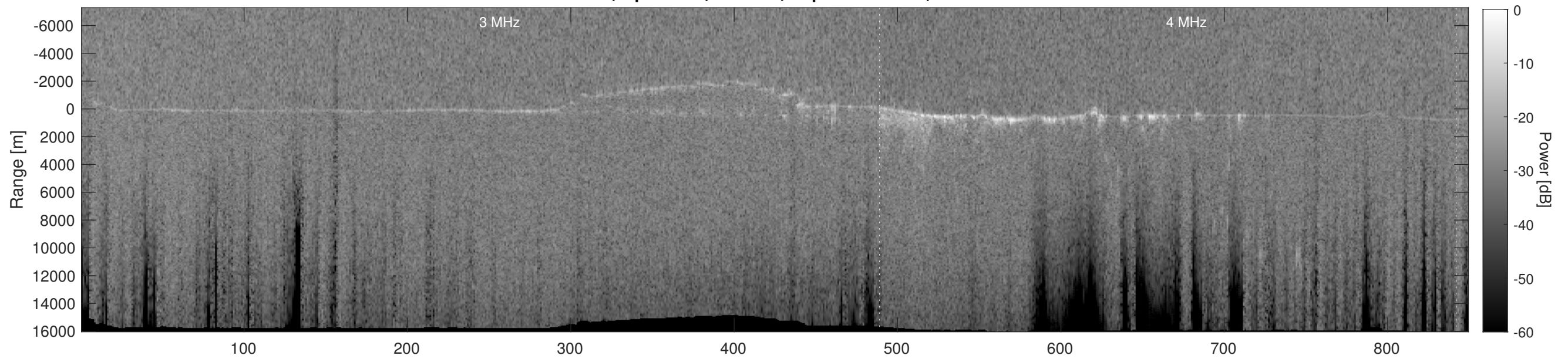
Orbit 9704, Depth-Corrected Cluttergram
