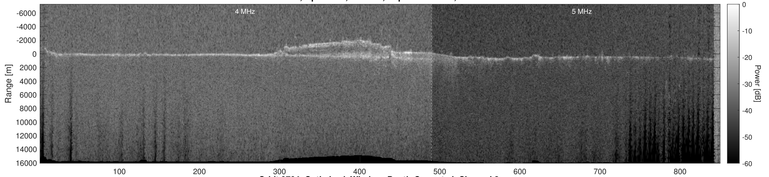
Orbit 9704, Optimized, Window, Depth-Corrected, Channel 2
