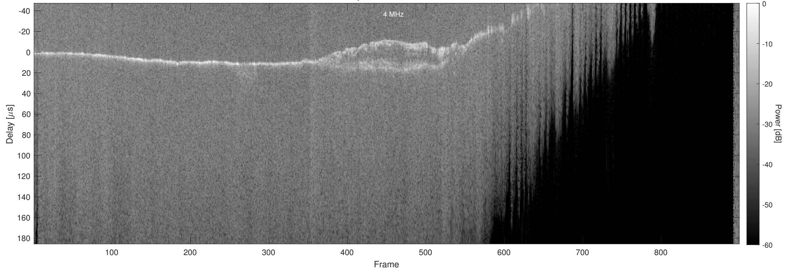
Orbit 9705, Chapman, No Window, Channel 2
