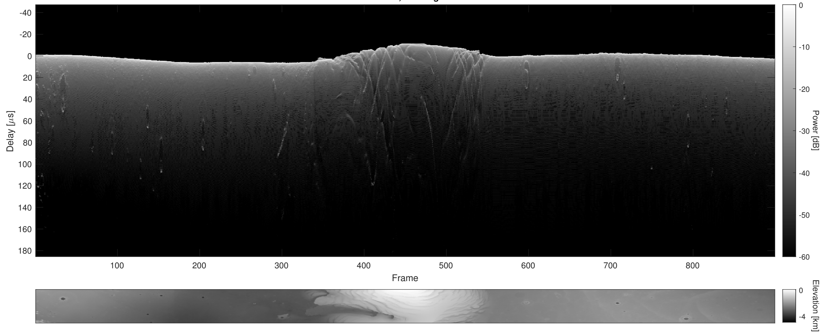
Orbit 9705, Cluttergram
