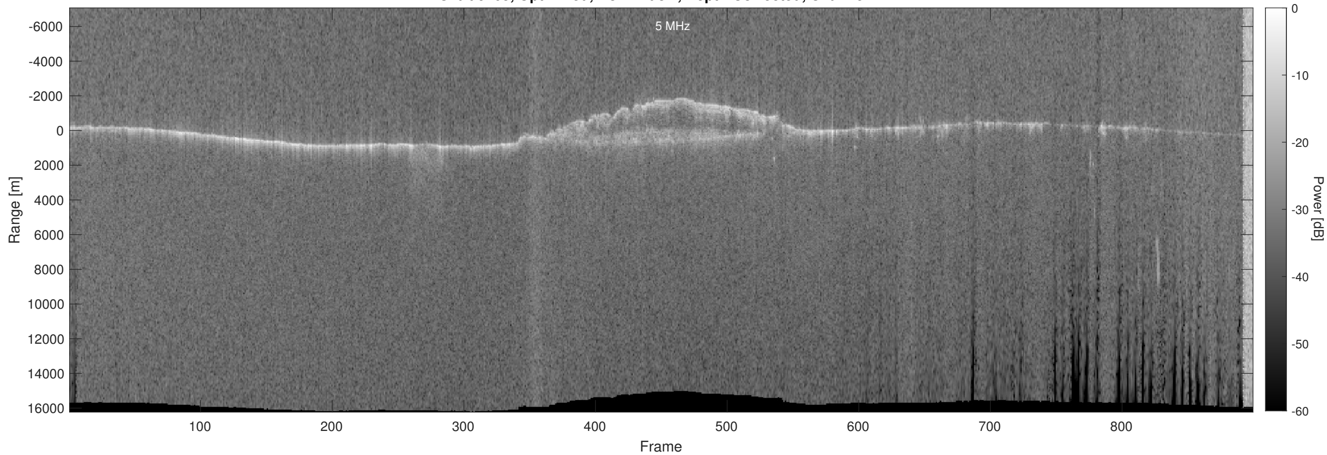
Orbit 9705, Optimized, No Window, Depth-Corrected, Channel 2
