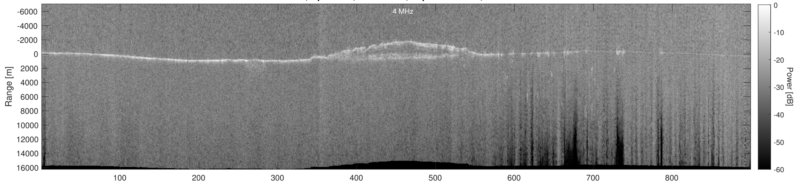
Orbit 9705, Depth-Corrected Cluttergram
