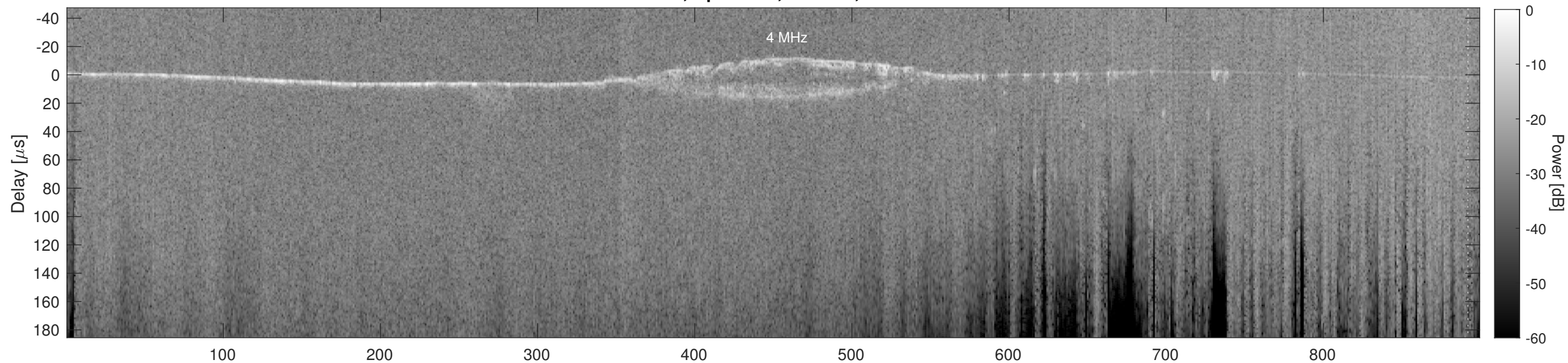
Orbit 9705, Cluttergram
