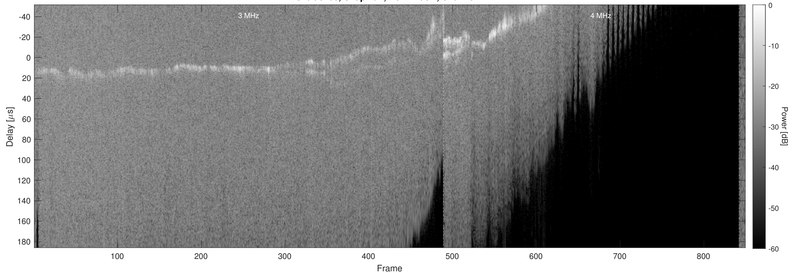
Orbit 9706, Chapman, No Window, Channel 2
