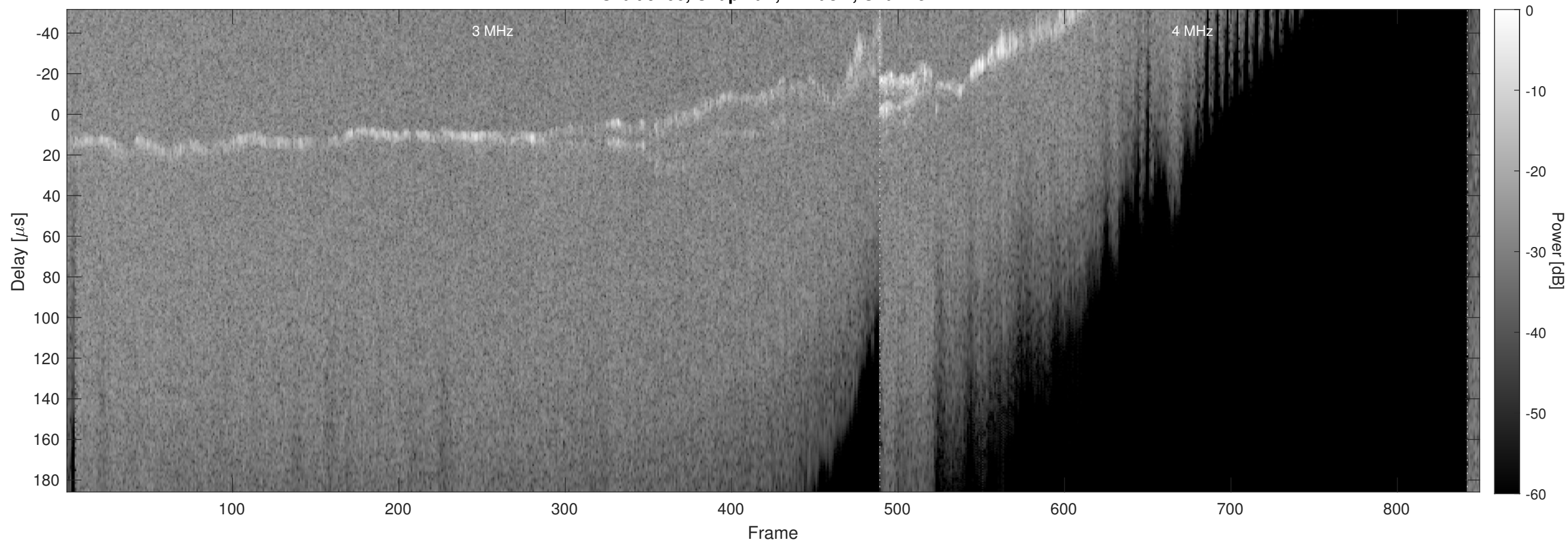
Orbit 9706, Chapman, Window, Channel 2
