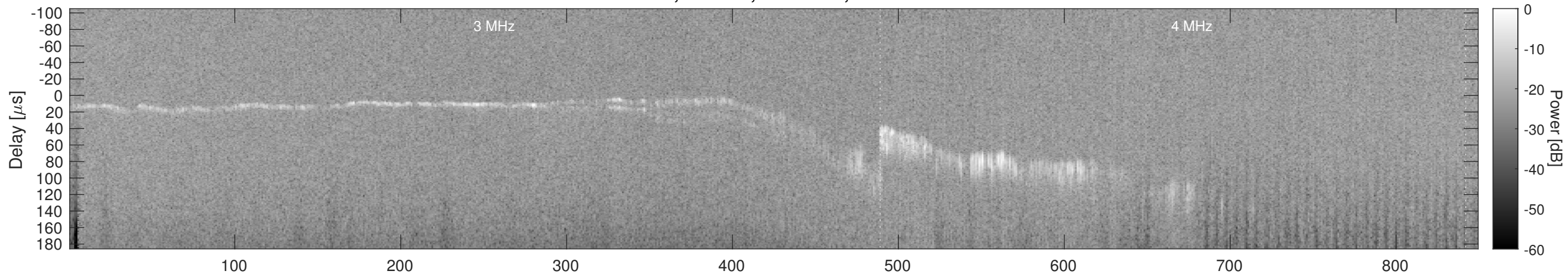
Orbit 9706, Window, Channel 2, Chapman
