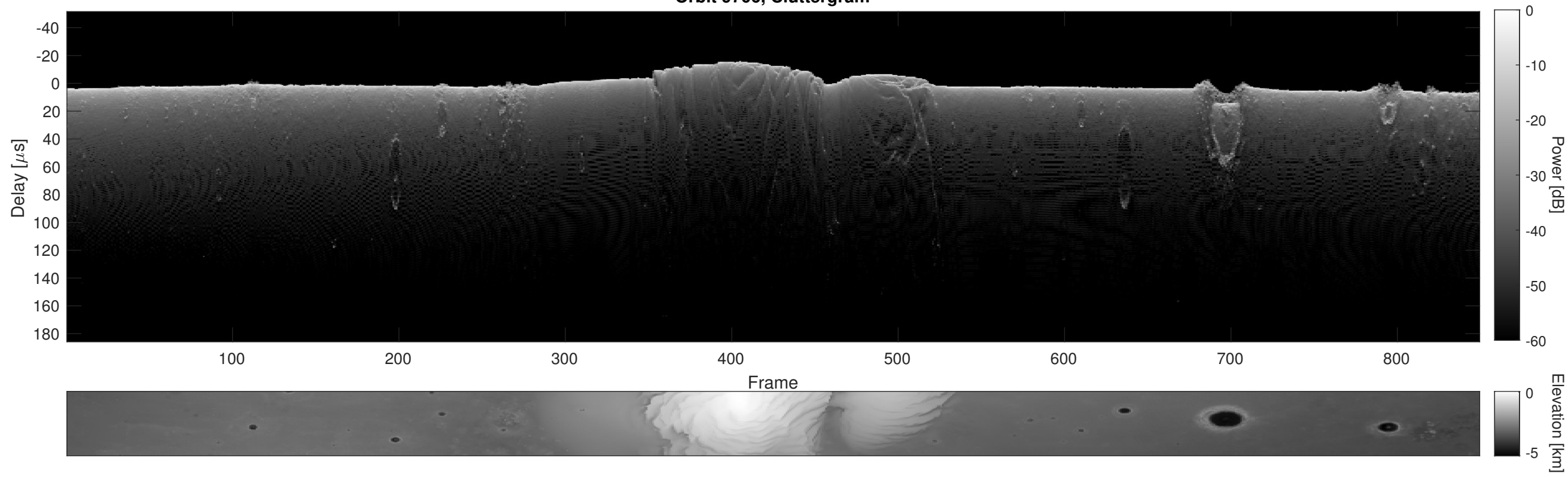
Orbit 9706, Cluttergram
