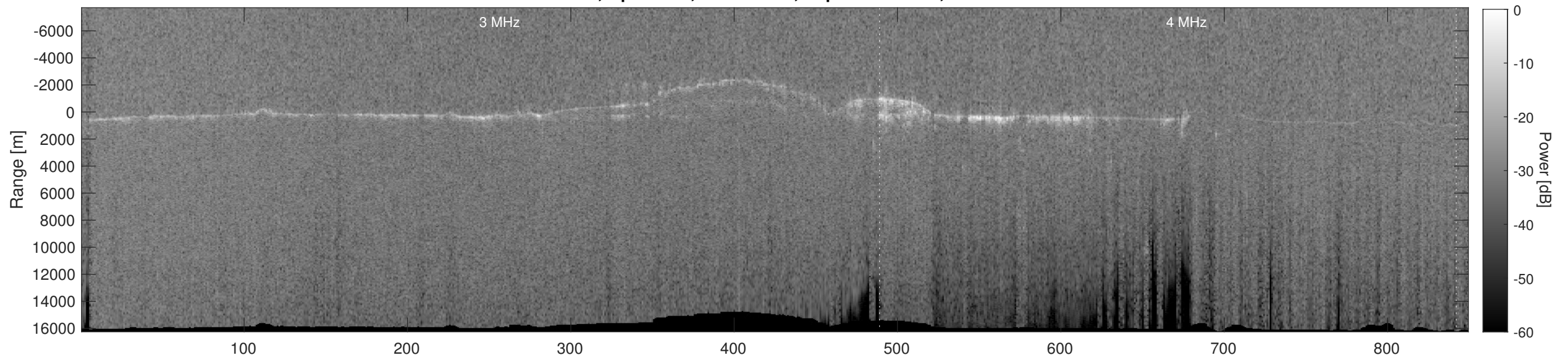
Orbit 9706, Depth-Corrected Cluttergram
