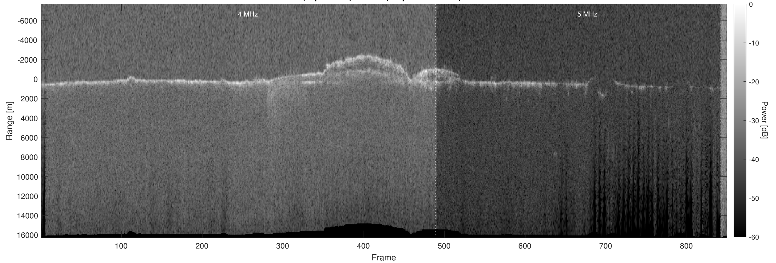
Orbit 9706, Optimized, Window, Depth-Corrected, Channel 2
