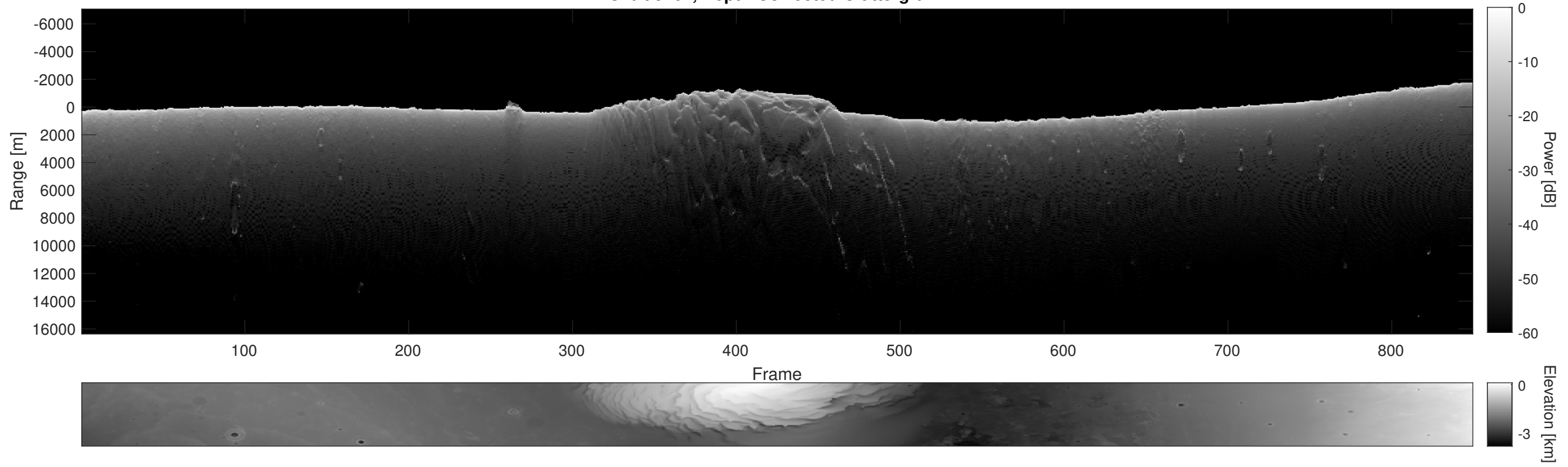
Orbit 9707, Depth-Corrected Cluttergram
