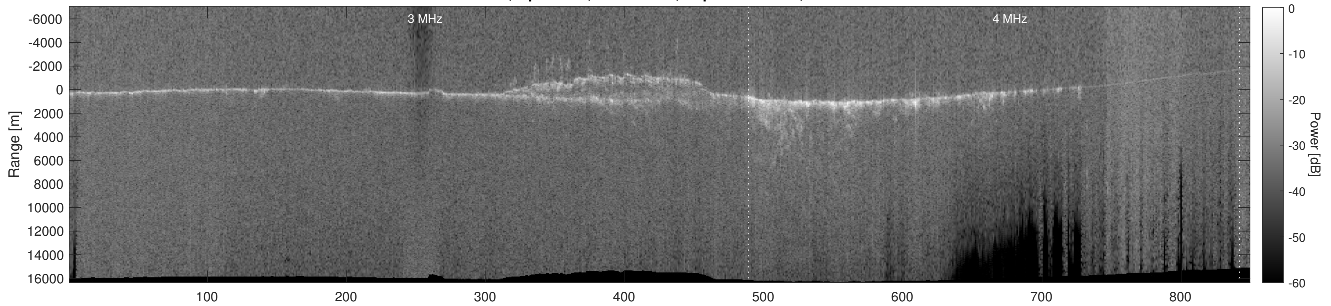
Orbit 9707, Depth-Corrected Cluttergram
