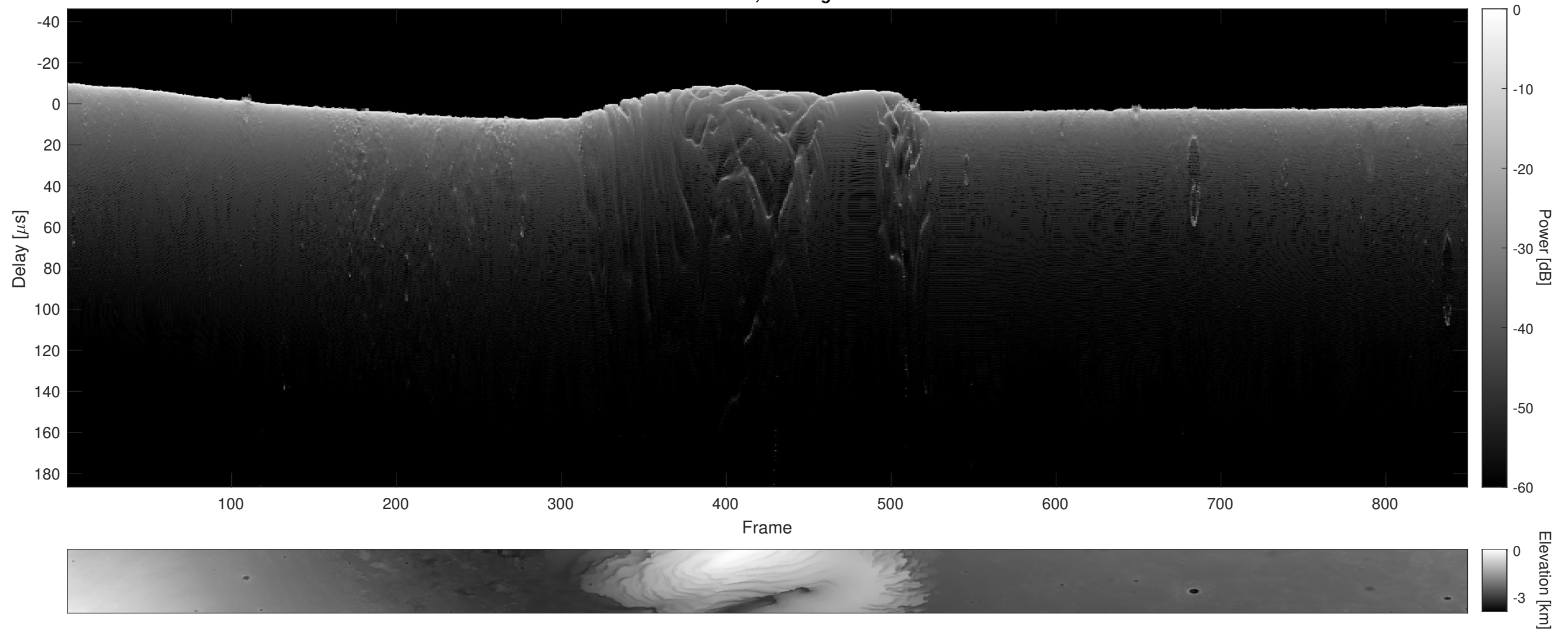
Orbit 9709, Cluttergram
