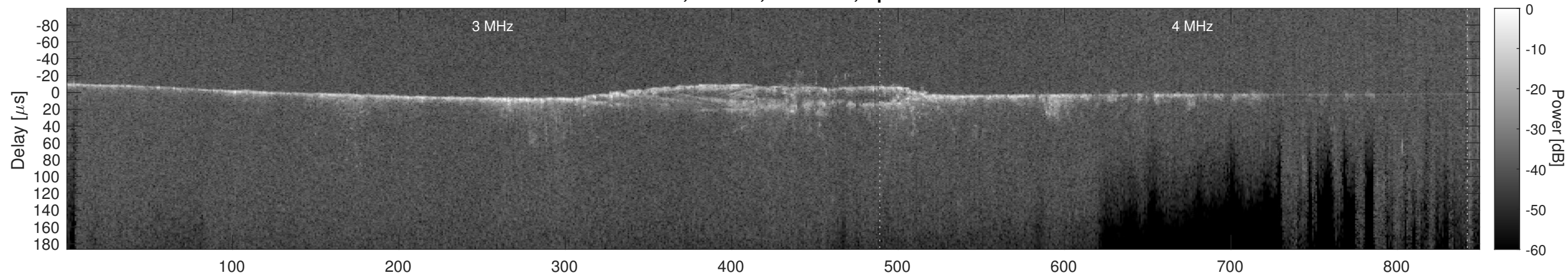
Orbit 9709, Cluttergram
