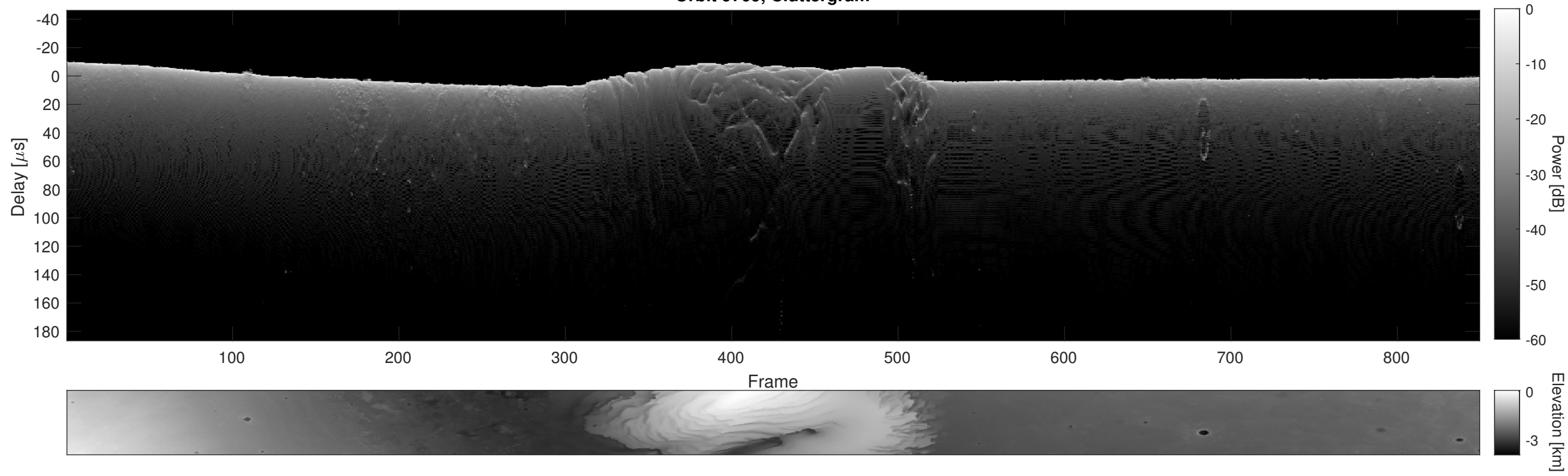
Orbit 9709, Cluttergram
