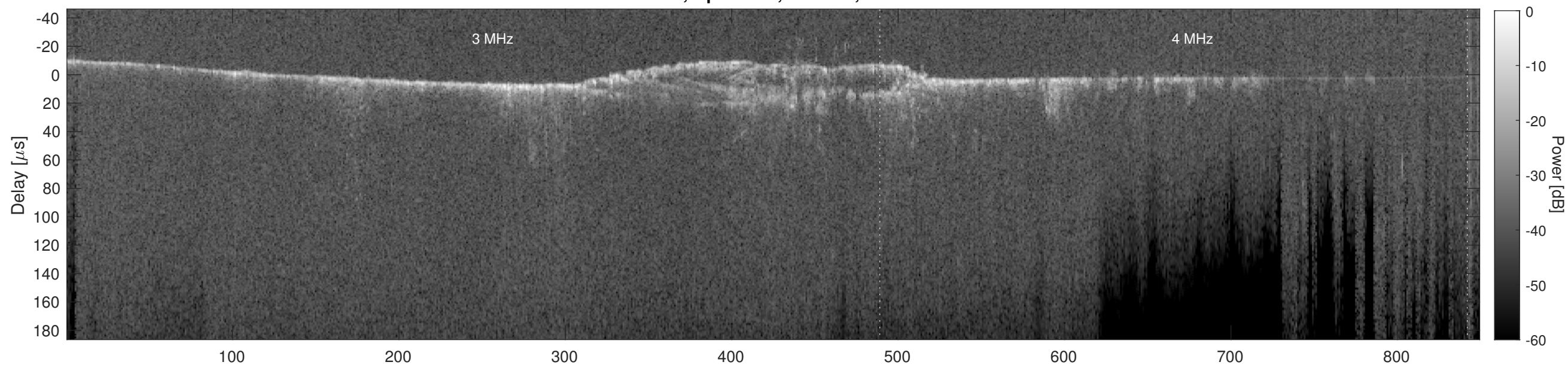
Orbit 9709, Cluttergram
