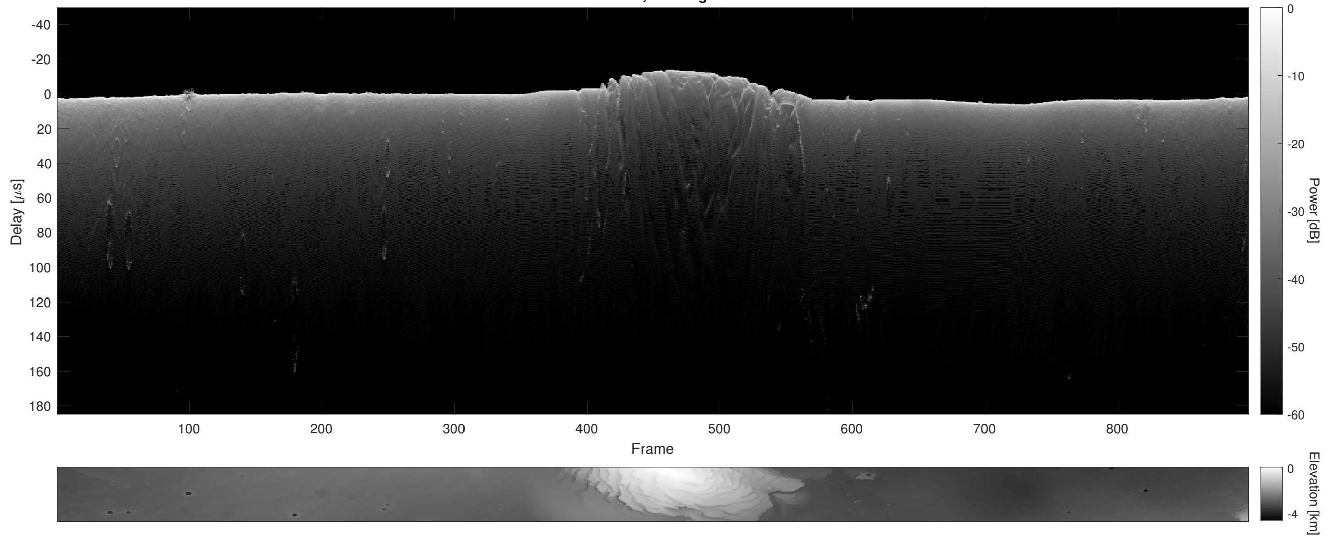
Orbit 9710, Cluttergram
