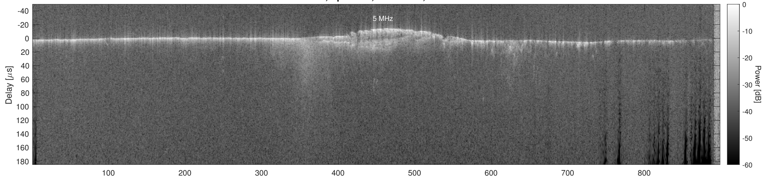
Orbit 9710, Optimized, No Window, Channel 2
