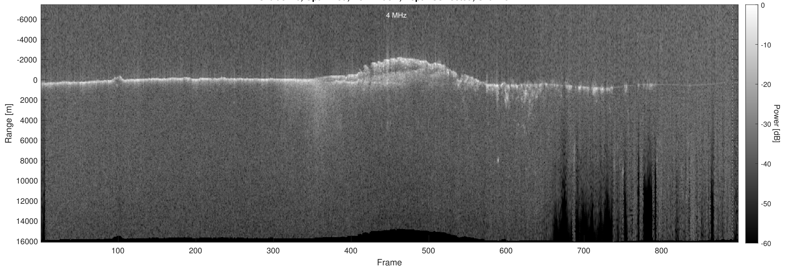
Orbit 9710, Optimized, No Window, Depth-Corrected, Channel 2
