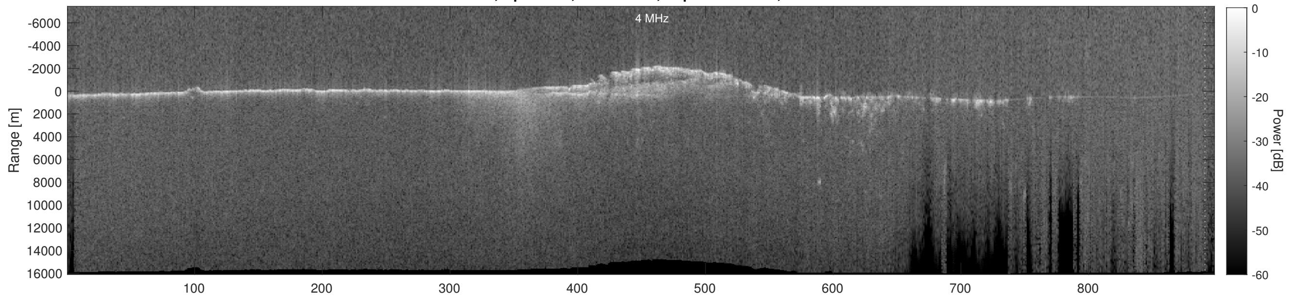
Orbit 9710, Depth-Corrected Cluttergram
