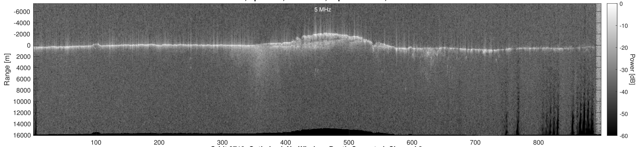
Orbit 9710, Optimized, No Window, Depth-Corrected, Channel 2
