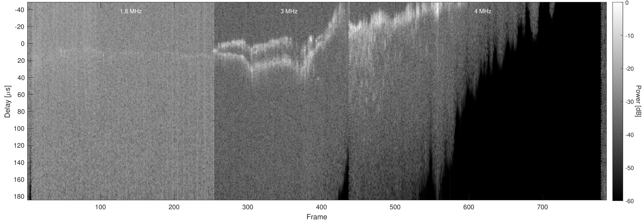
Orbit 9711, Chapman, No Window, Channel 2
