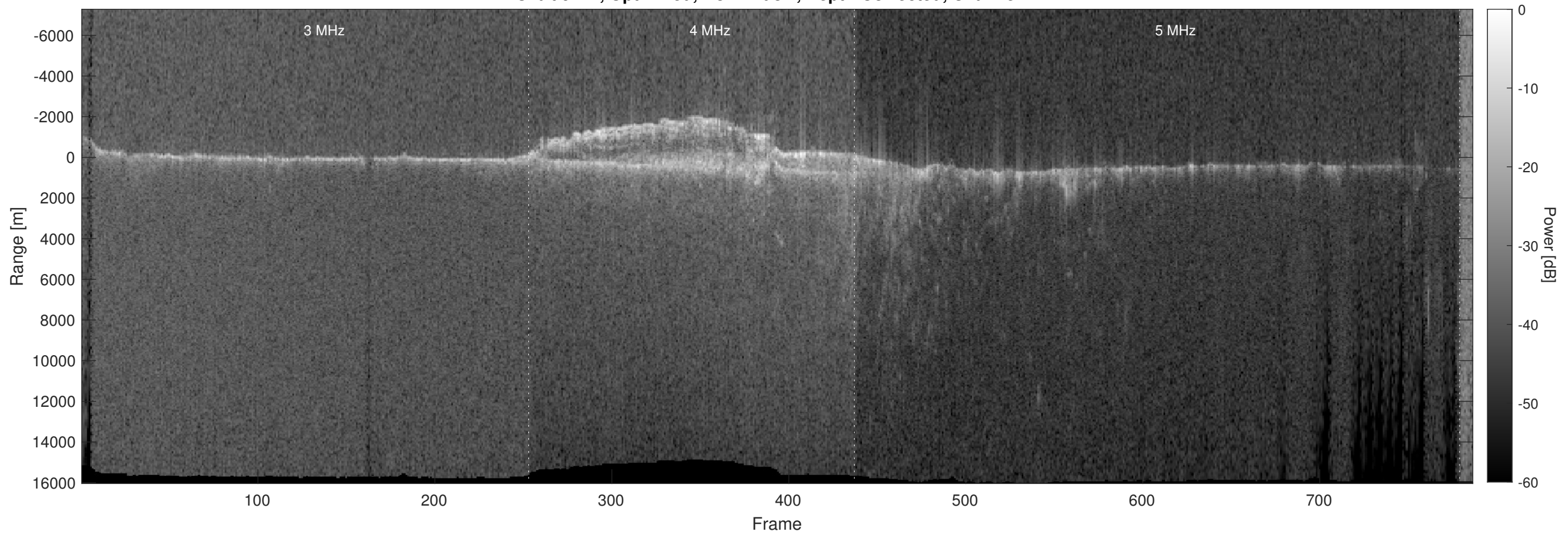
Orbit 9711, Optimized, No Window, Depth-Corrected, Channel 2
