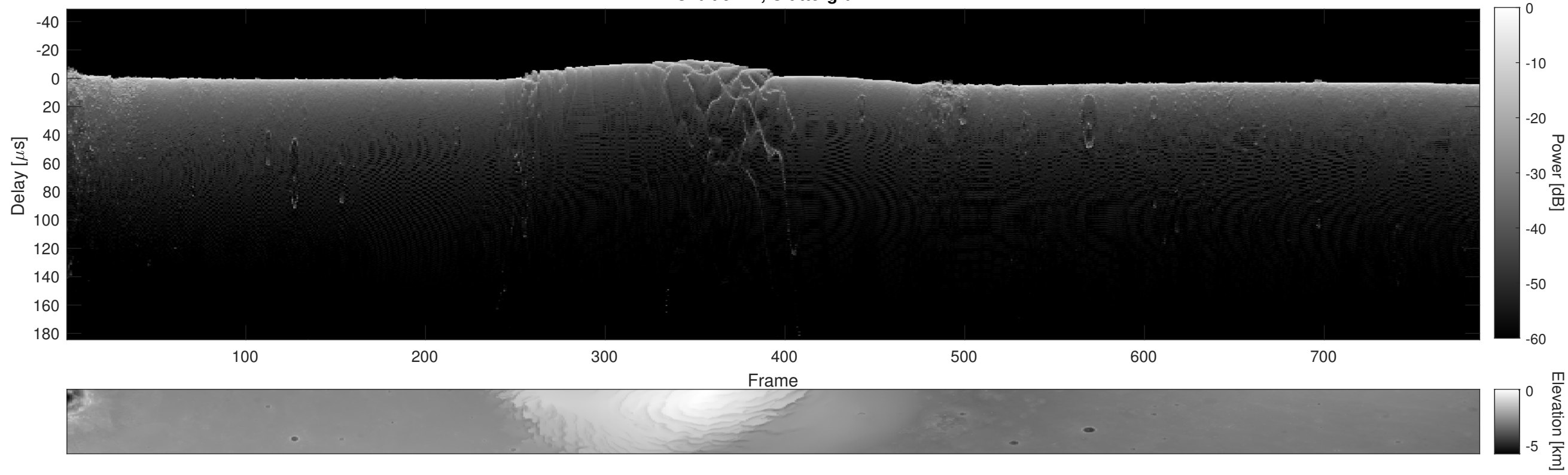
Orbit 9711, Cluttergram
