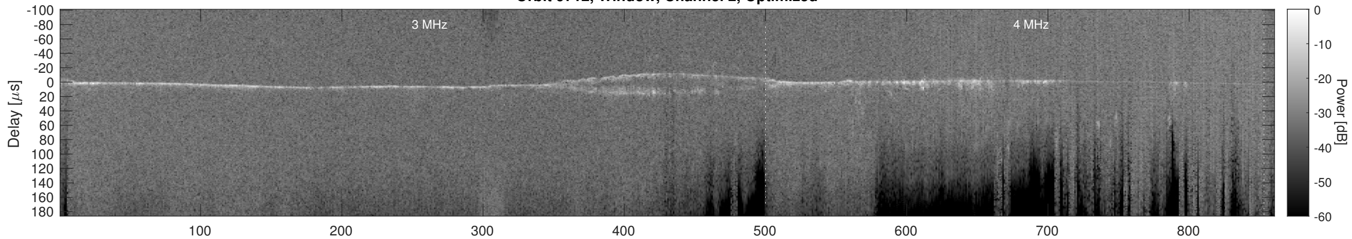
Orbit 9712, Cluttergram
