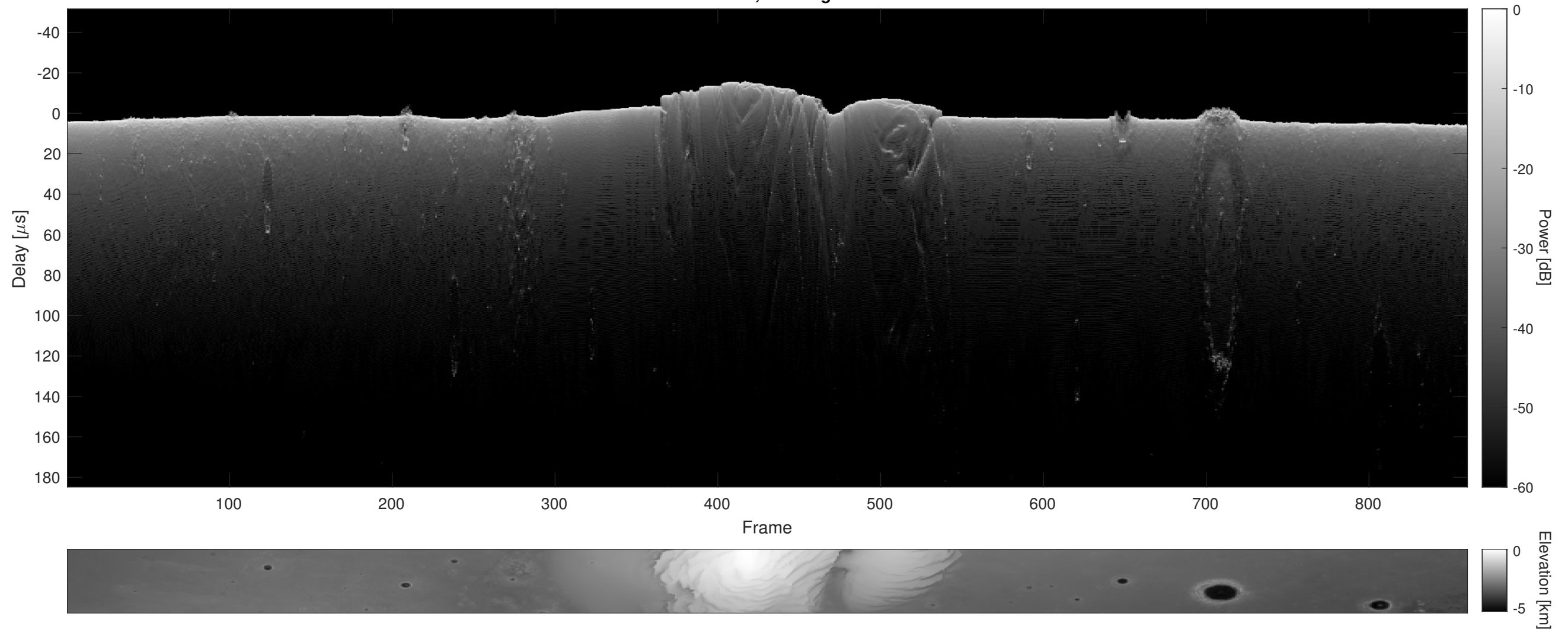
Orbit 9713, Cluttergram
