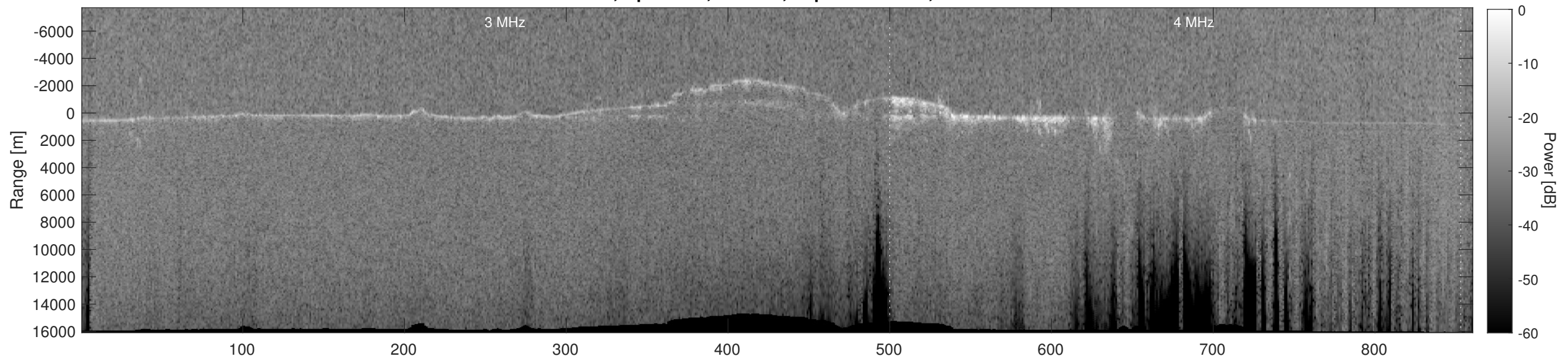
Orbit 9713, Depth-Corrected Cluttergram
