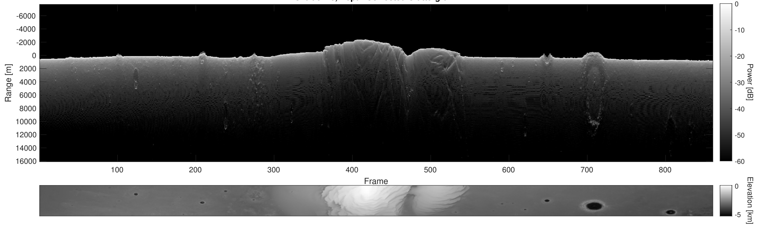
Orbit 9713, Depth-Corrected Cluttergram
